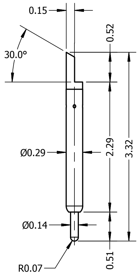
PIN CONTACT DETAIL SCALE 25 : 1 CS1512-T2
