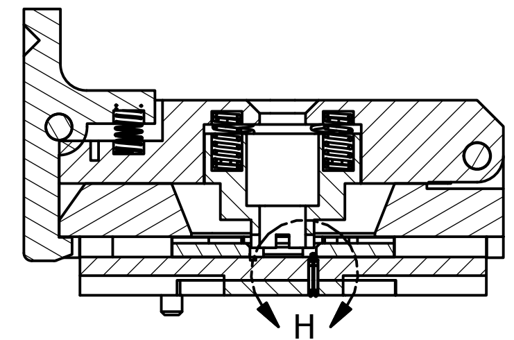
SECTION G-G SCALE 2.5 : 1
