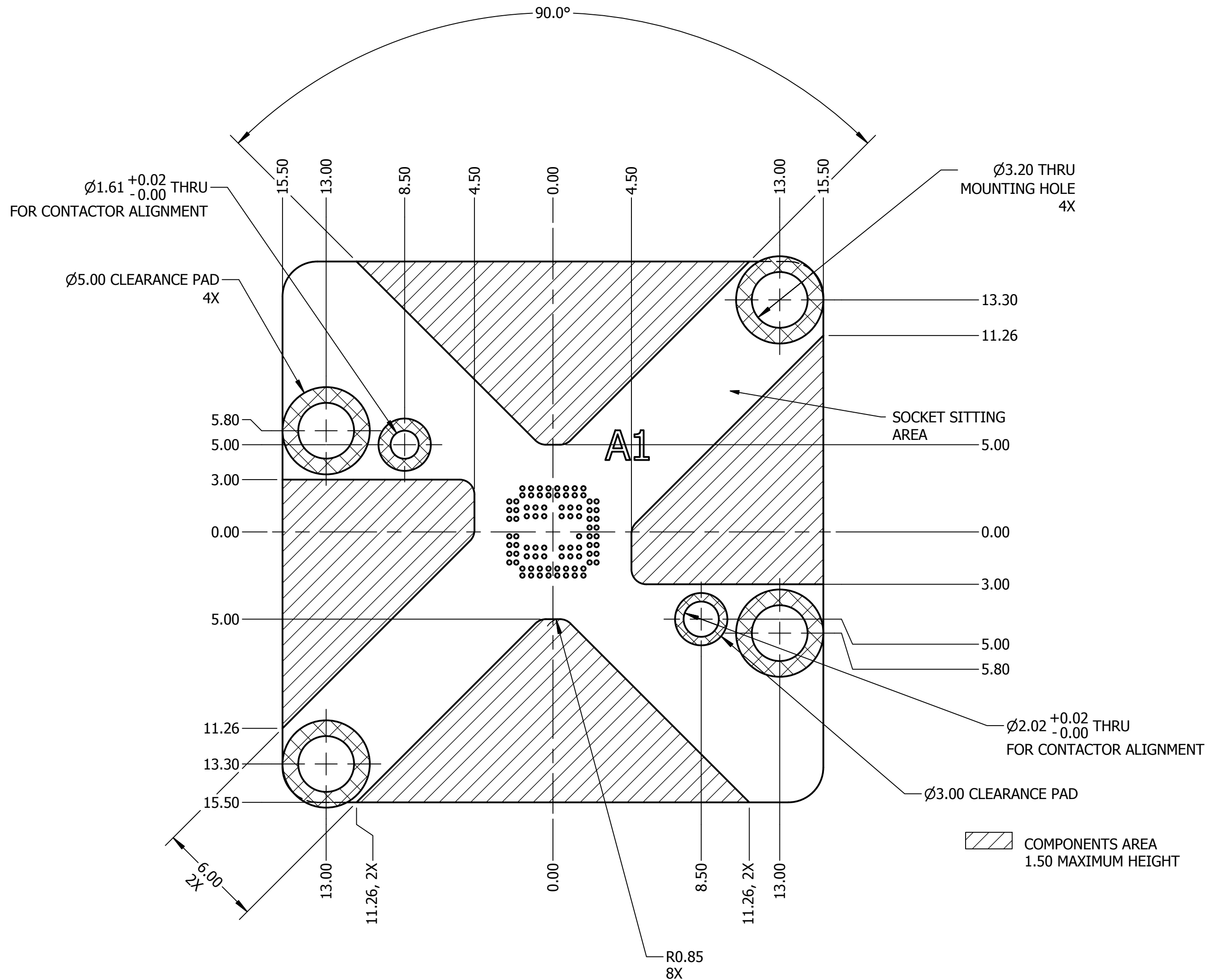
TOP VIEW SCALE 5 : 1
