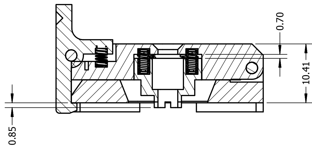
SECTION F-F SCALE 2.5
