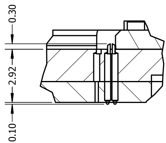
DETAIL C SCALE 8 : 1
