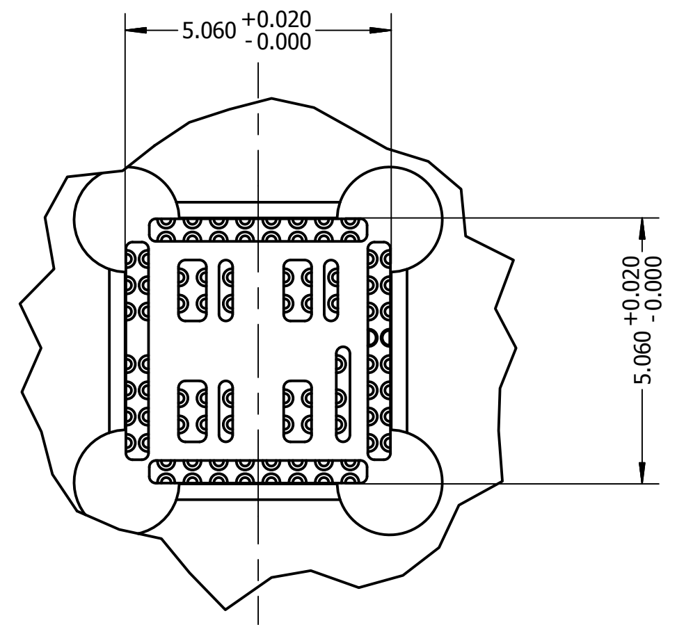
DETAIL E SCALE 10: 1
