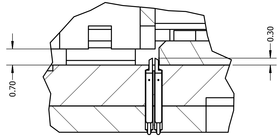
DETAIL H SCALE 12 : 1
