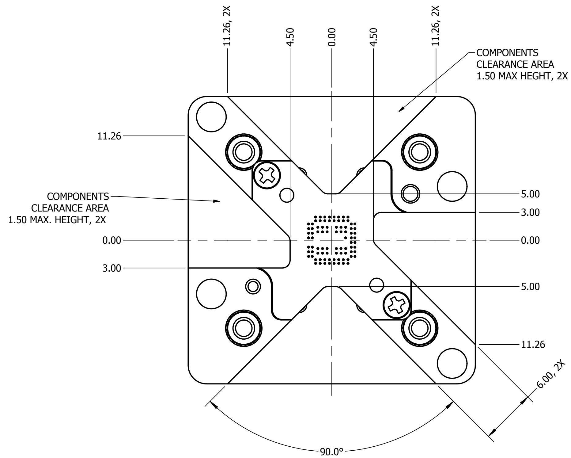
BOTTOM VIEW SCALE 4 : 1
