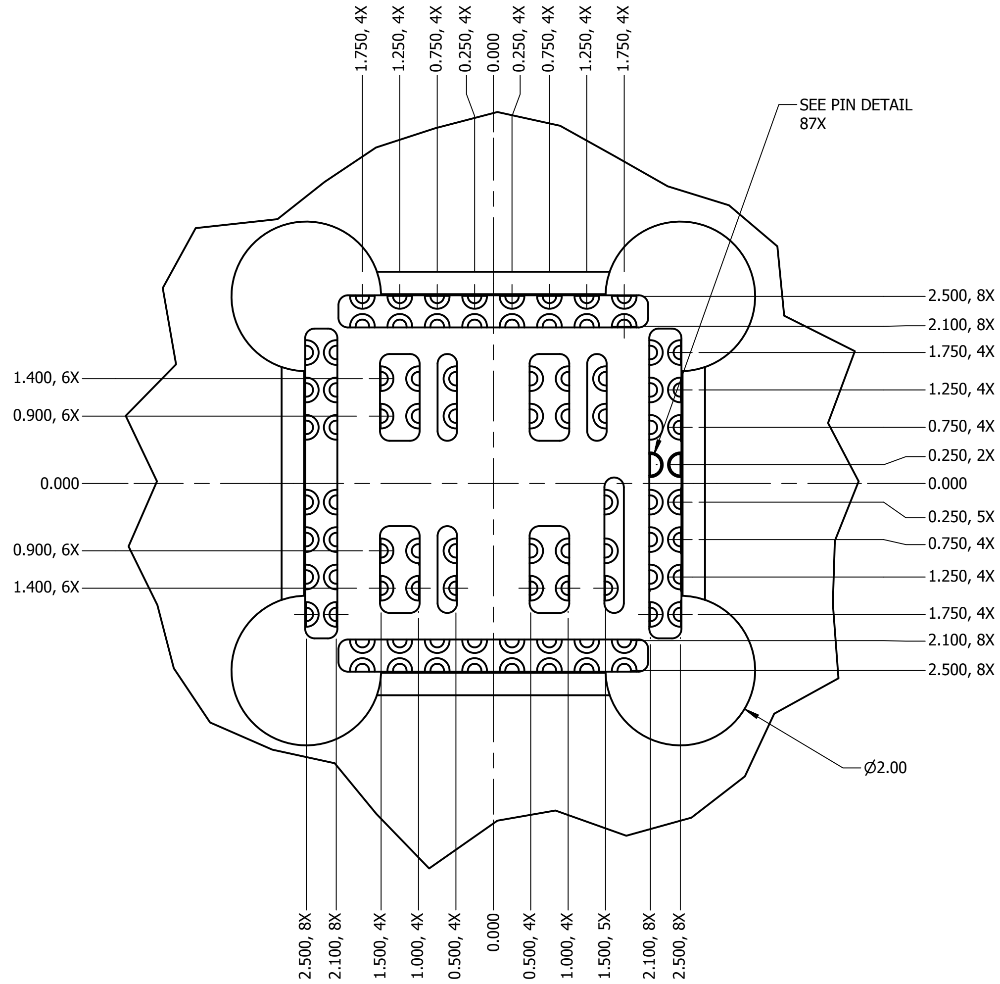
DETAIL F SCALE 20: 1
