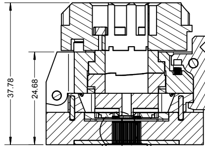
SECTION H-H SCALE 2: 1
