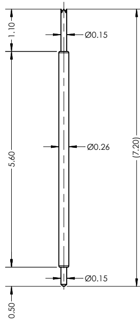
CONTACT DETAIL SCALE 20 : 1
