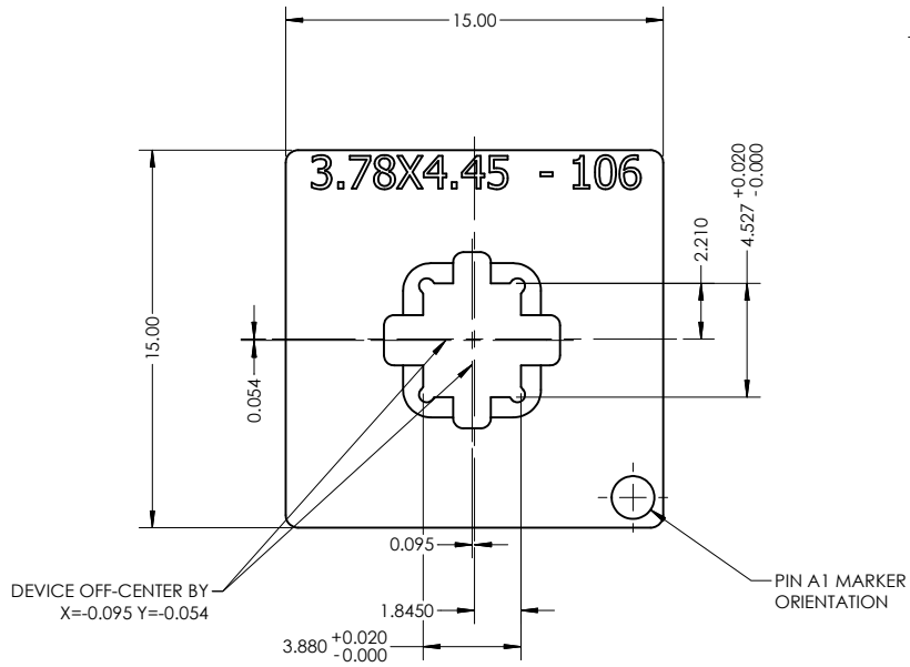
TOP VIEW SCALE 6 : 1
