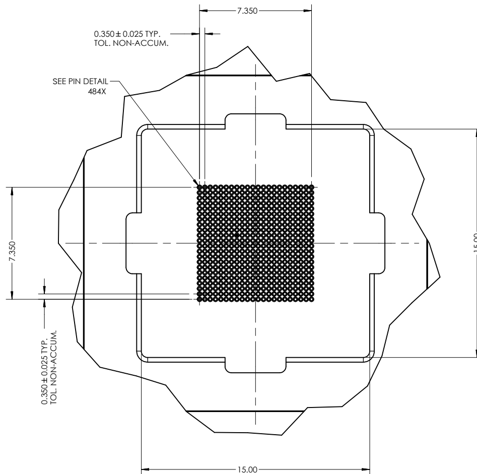
DETAIL B SCALE 8 : 1
