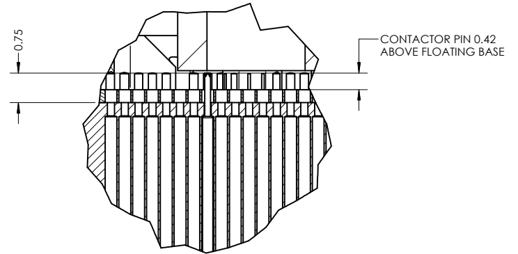
DETAIL L SCALE 15: 1
