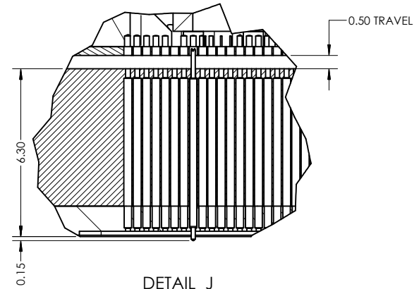
DETAIL J SCALE 10: 1
